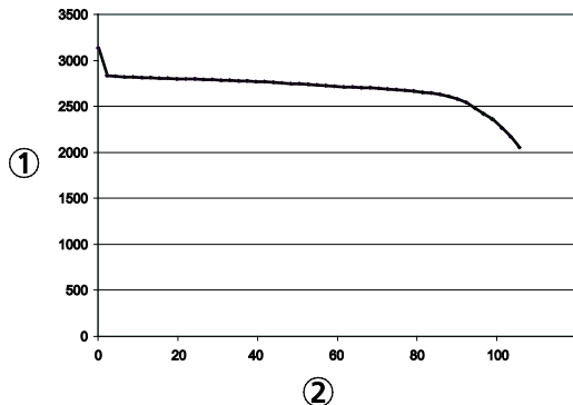
Figure 3. Battery Discharge Curve
